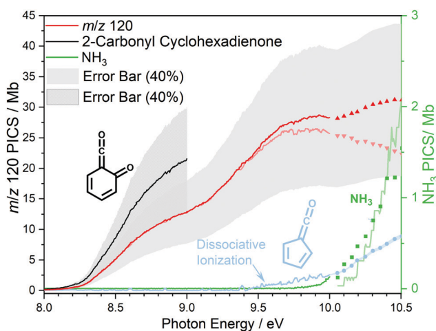
Fig. 5 The lumped photoionization cross section (red curve) of the m/z 120 species 2-carbonyl cyclohexadienone 2 and benzpropiolactone 6 along with the fulvenone fragment (blue curve). Effective PICS of the ketoketene 2 is depicted in black. We assume a conservative error bar of 40%.
