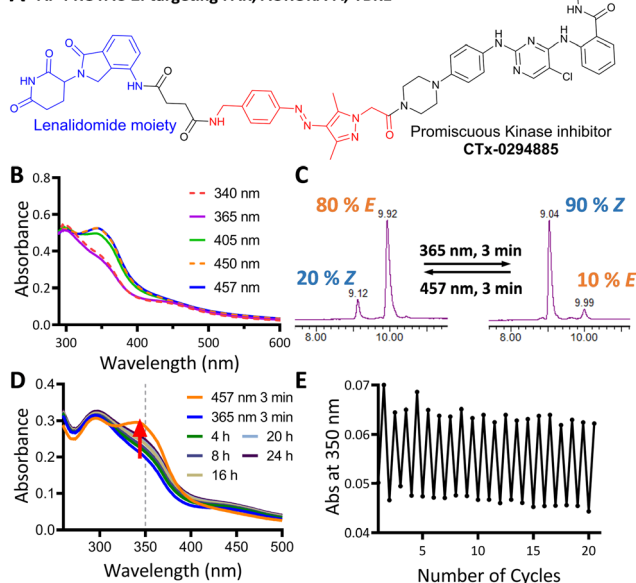
Fig. 3 (A) Structure of Photoswitchable multi-kinase targeting degrader AP-PROTAC-2. (B) UV-Vis spectra of 20 \mu M AP-PROTAC-2 in water with 0.2% DMSO with 3 min irradiation. (C) LC-MS chromatograms of 0.1 mM AP-PROTAC-2 in 20% acetonitrile in water under the stated irradiation conditions. (D) UV-Vis spectra of 12 \mu M AP-PROTAC-2 in water with 0.1% DMSO after 365 nm irradiation recorded over time at 37 ^{\circ} C. (E) Reversible switching of 10 \mu M AP-PROTAC-2 solution in water with 0.1% DMSO at RT following 365 nm or 457 nm irradiation for 20 cycles.
