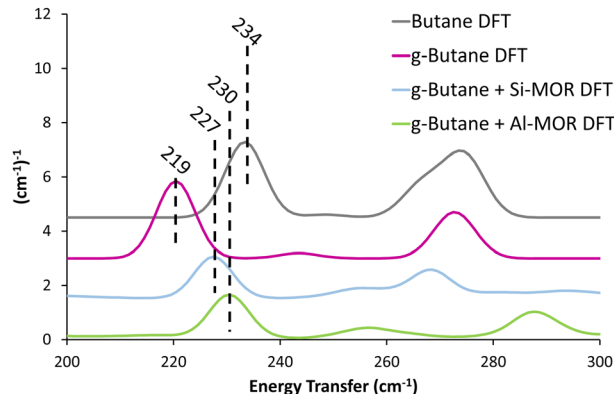
Fig. 3 Calculated INS spectra of unconstrained antiperiplanar n -butane (Butane DFT) and gauche distorted butane unconstrained (g-Butane DFT), within siliceous (Si-MOR) and acidic (Al-MOR) mordenite pores shows the deviation in the methyl torsion peak position between the conformers, akin to the experimental findings (Fig. 1). Spectra are artificially shifted by 1.5 (\text{cm}^{-1})^{-1} for ease of reading.
