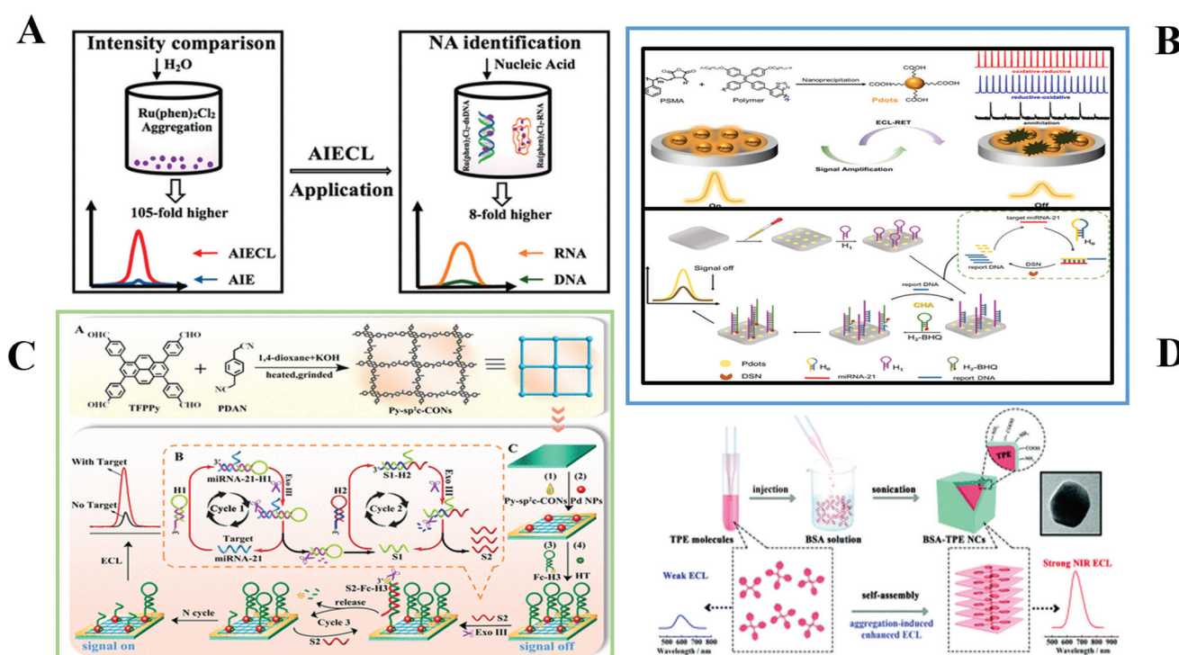
Fig. 7 AIECL of the (Ru(phen) 2 Cl 2 )/TPA system and its applications. Adapted from (Lu et al. 2020) with permission of Analytical Chemistry , copyright 2020 (A). Synthesis of active Pdts and the preparation of a sensor for miRNA-21. Adapted from (Zhang et al. 2021) with permission of Analytical Chemistry , copyright 2021 (B). Construction of a Py-sp 2 c-CON emitter and a designed sensor for microRNA-21. Adapted from (Zhang et al. 2021) with permission of Analytical Chemistry , copyright 2021 (C). Assembly process of a sensor for microRNA. Adapted from (Liu et al. 2019) with permission of Analytical Chemistry , copyright 2019 (D).
