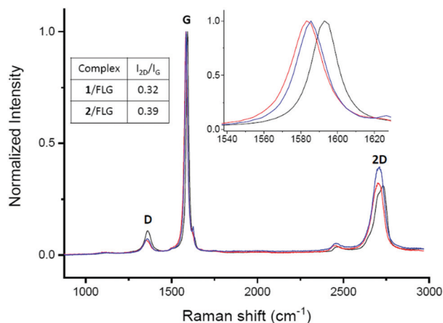
Fig. 2 Raman spectra ( \lambda_{\text{exc}} = 532 nm) of FLG (black) and its complexes with 1 (red) and 2 (blue).
