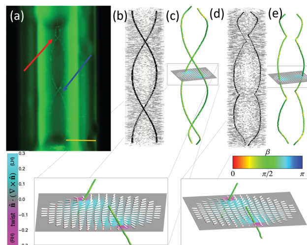
Fig. 2 (a) Fluorescent amphiphile BODIPY-C5 with CCN-47 mixture. Fluorescent molecules accumulate at the defects in the twisting disclination lines. As the escaped radial configuration onsets, the end of the disclination line forms a twisted loop. Scale bar 20\text{ }\mu\text{m} . (b and d) Computer simulated LCs in round capillaries with different elastic anisotropy, forming either a regular helical structure (b) or a lozenge-like structure (d). The elastic anisotropy in (b) is K_2/K_3 = 0.2 while in (d) it is K_2/K_3 = 0.13 . In all cases, K_1 = K_3 = 10^{-11}\text{ N} . The simulation size corresponds to a capillary with circular cross section, radius 112.5\text{ nm} and length 675\text{ nm} . The capillary walls impose strong homeotropic anchoring while the top and bottom are modeled as very weak degenerate planar anchoring. The black lines show the defect lines and the gray glyphs the nematic director. (c and e) The twist/wedge character of the twisted defect lines plotted in b and d respectively. The winding type of the disclination is mostly twist (green) but shows an intermediate character (yellow) especially close to the kinks (e). The expanded details show the nematic director on one plane between two twist lines.
