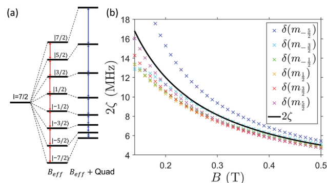
Fig. 5 (a) Schematic representation of the energy-levels splitting of an I = 7/2 spin in presence of an effective field B_{\text{eff}} and with the addition of a quadrupole coupling, making the gaps inequivalent (note that the effect of quadrupole is here exaggerated for clarity). (b) Difference between the energy gap of consecutive nuclear transitions \delta(m_I) = (E_{m_I+1} - E_{m_I}) - (E_{m_I} - E_{m_I-1}) in the m_S = -1/2 subspace, as a function of static field, applied along x . Results from diagonalization of the effective rank-2 pseudo-quadrupolar Hamiltonian (2) are shown in black, in very good agreement with results from exact diagonalization of the full Hamiltonian (1) (colored crosses), especially at large B_0 .
