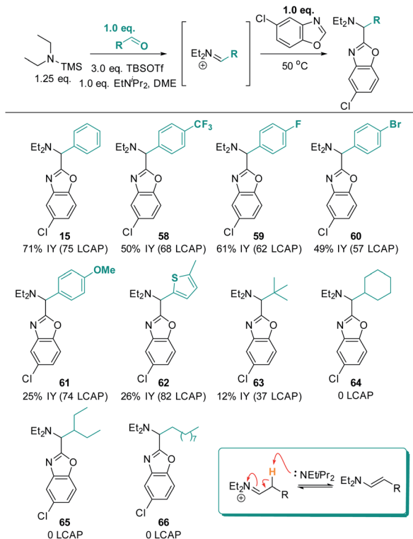
Scheme 16 Aldehyde scope. Conditions: azole (1.0 eq.), TBSOTf (0.416 mL, 1.813 mmol, 3.0 eq.), \text{TMS}-\text{NEt}_2 (1.25 eq.), \text{PhCHO} (1.0 equiv.), \text{EtN}^i\text{Pr}_2 (1.0 equiv.), \text{N}_2 , 50 °C, 18 h.
