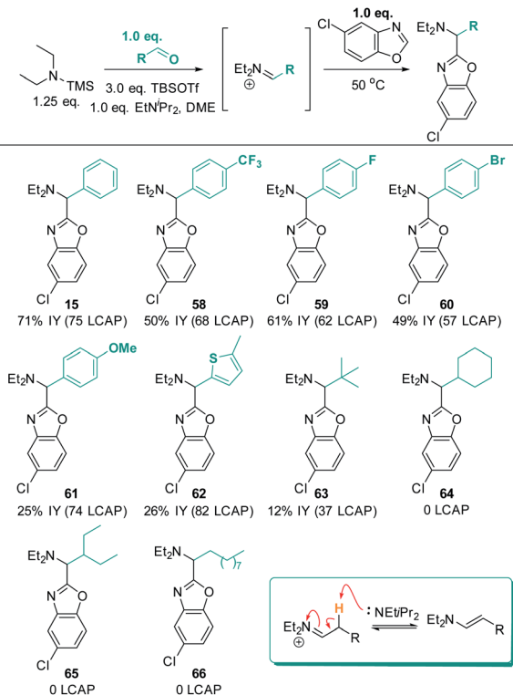
Scheme 16 Aldehyde scope. Conditions: azole (1.0 eq.), TBSOTf (0.416 mL, 1.813 mmol, 3.0 eq.), TMS–NEt 2 (1.25 eq.), PhCHO (1.0 equiv.), Et 3 NPr 2 (1.0 equiv.), N 2 , 50 °C, 18 h.
