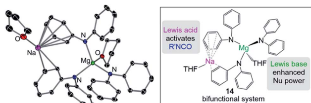
Fig. 3 Molecular structures of alkali-metal magnesiate [(\text{THF})\text{NaMg}(\text{NPh}_2)_3(\text{THF})] ( 14 ).
