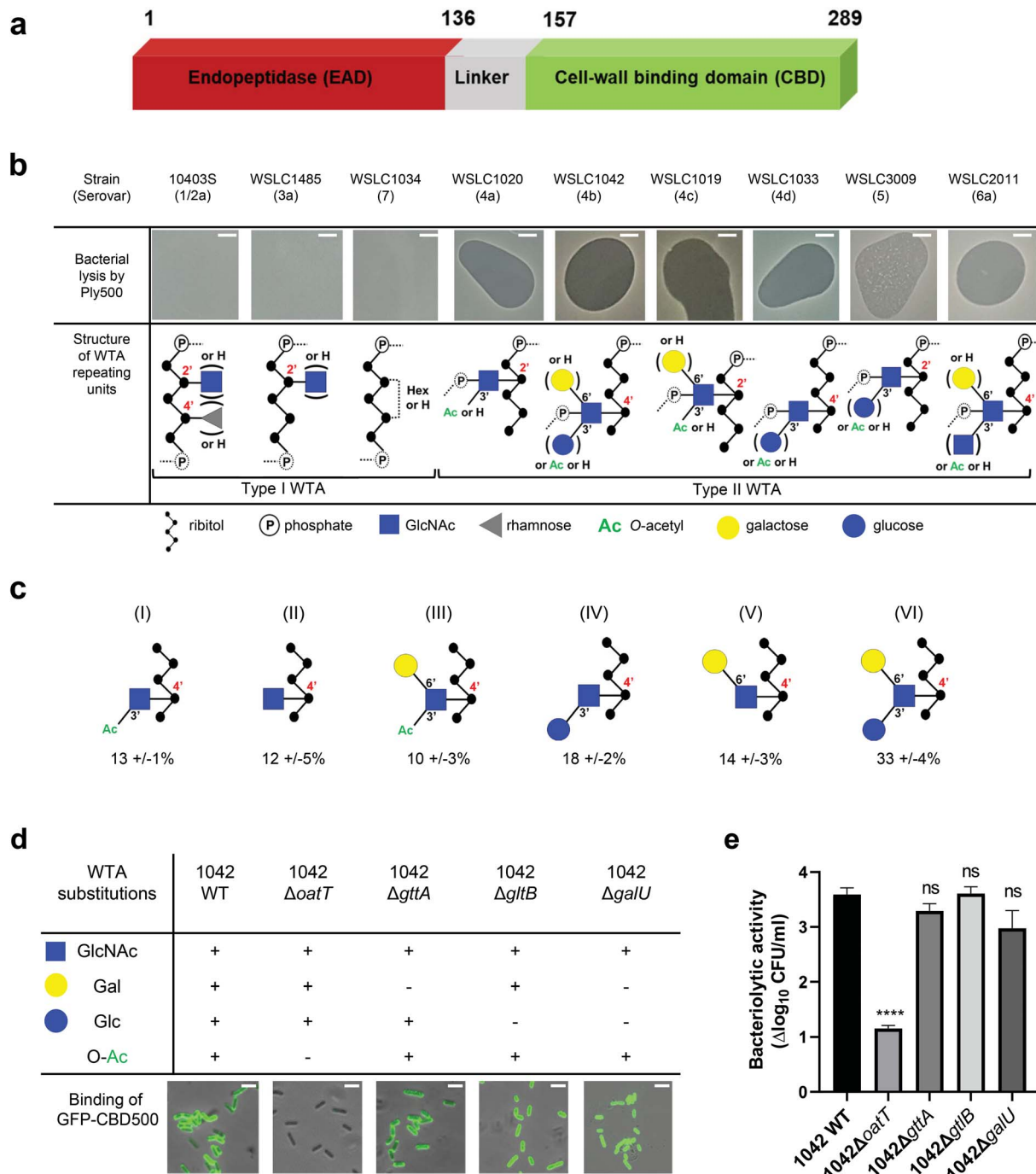
Fig. 1 Correlation of Listeria WTA structure with the bacteriolytic activity of Ply500 endolysin and the binding activity of its C-terminal domain CBD500. (a) Modular architecture of the full-length Ply500. (b) Lytic activity of Ply500 detected by spot-on-lawn assay (upper panel; scale bar 300 \mu m) and corresponding types of WTA reported in the genus Listeria . 20 Images are representative of three experiments, and contrast was adjusted for clarity. (c) Relative abundance (%) of the repeating unit variants within Listeria WTAs derived from strain WSLC1042 (WTA 1042 ), determined by UPLC-MS analysis. Latin numerals (I–VI) denote the repeating unit species of WTA 1042 identified. Data represent means \pm SEM; n = 3 . (d) Binding of GFP-CBD500 to wild-type WSLC1042 and mutants lacking specific substituents in the backbone of the WTA repeating unit. Scale bar represents 1 \mu m. Images are representative of three experiments, and contrast was adjusted for clarity. (e) Reduction of bacterial colony counts ( \Delta \log_{10} CFU ml -1 ) after 1 h incubation of WSLC1042 and selected WTA mutants in the presence of 100 \mu g ml -1 of Ply500. Results are the mean \pm SEM of three experiments. Statistical significance was assessed using one-way ANOVA test (**** p < 0.0001 ; ns: not significant).
