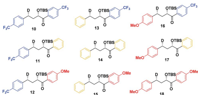
Fig. 5 syn substrates for a NY-II reaction.
