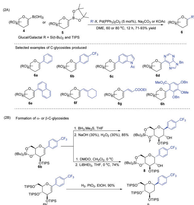
Scheme 2 (A) Aryl or heteroaryl or alkenyl-C-glycols using Suzuki-Miyaura cross-coupling and (B) formation of the corresponding α- & β-C-glycosides.
