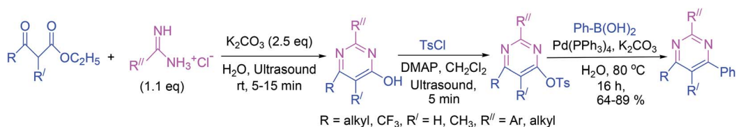
Scheme 16 Synthesis of 4-arylpuridines under ultrasound irradiation.
