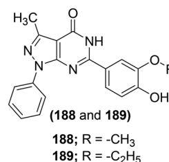
Fig. 61 Chemical structures of selected pyrazolopyrimidines (188 and 189).
