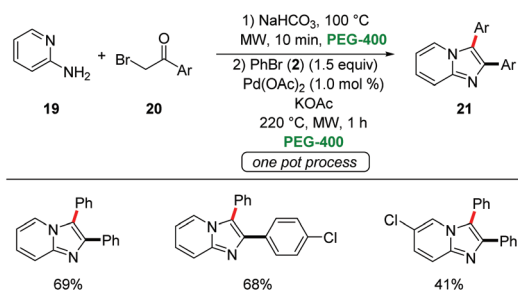
Scheme 5 One pot sequential approach for palladium-catalyzed arylation in PEG-400.
