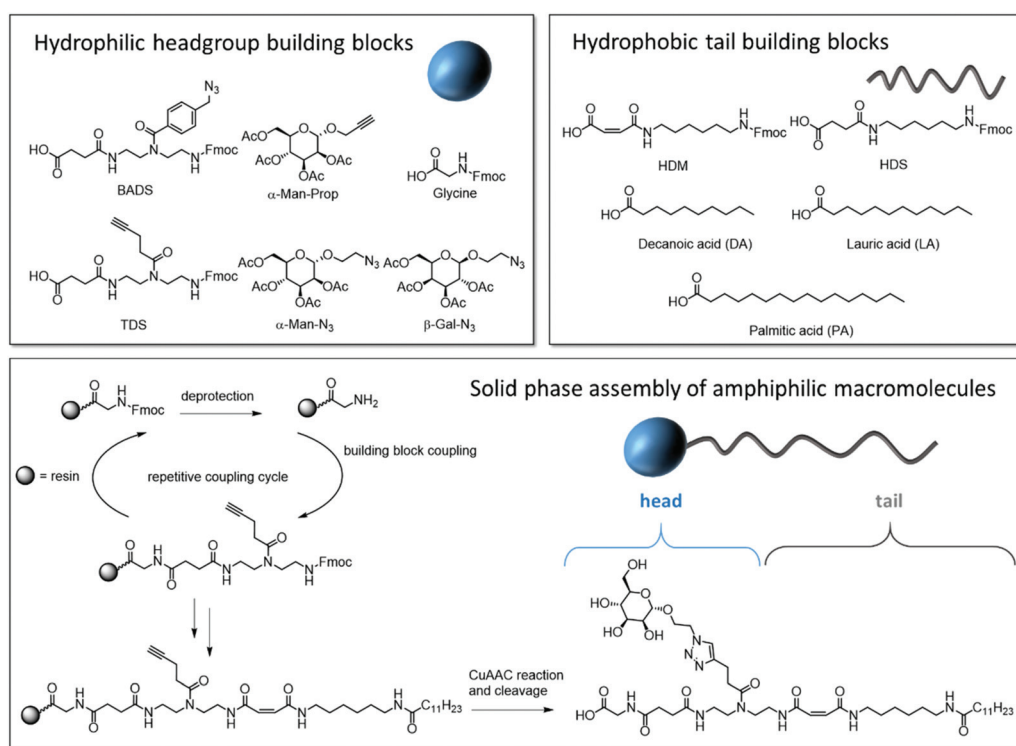
Fig. 1 Overview of the utilized building blocks and their position in the APG, general solid phase synthesis of APGs exemplarily shown for structure 1 (Gly-TDS(Man)-HDM-C12).
