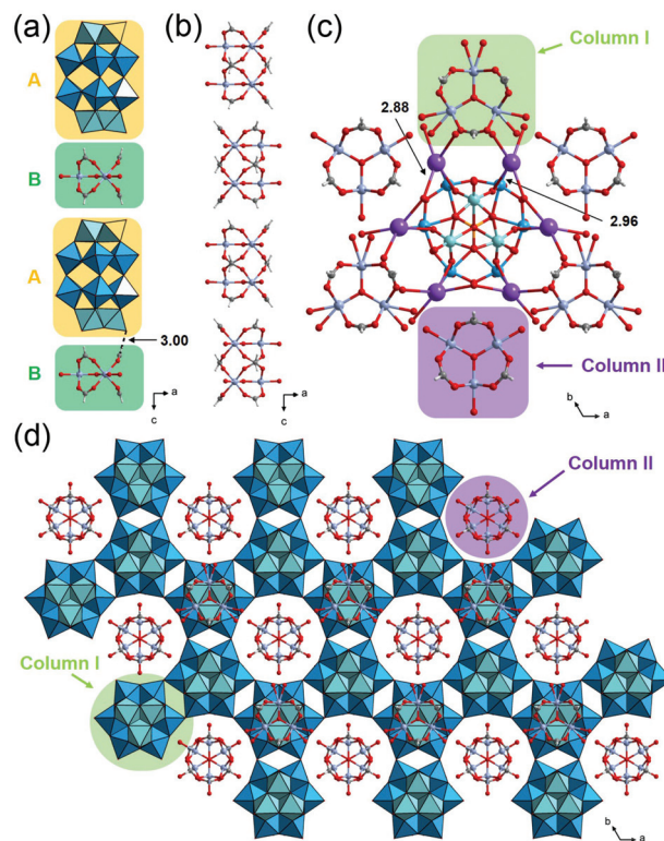
Fig. 3 Crystal structure of K_5[Cr_3O(OOCH)_6(H_2O)_3]_2[P_2W_{15}Nb_3O_{62}] \cdot 18H_2O ( 2 ). Color codes are the same as Fig. 2. (a) Arrangement of a POM and macrocation in column I. (b) Arrangement of a macrocation in column II. (c) Local view of a POM and the surrounding K^+ ions and macrocations. (d) Honeycomb-like lattice.
