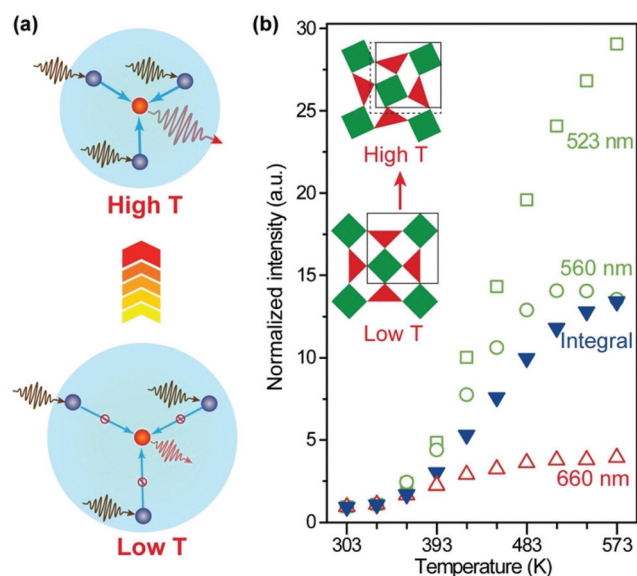
Fig. 7 (a) Thermal promotion of energy delivery to activator ions by lattice contraction in negative thermal expansion crystals. (b) Normalized emission intensities of \text{Yb}_2\text{W}_3\text{O}_{12}:\text{Er} (6%) nanocrystals as a function of temperature. Inset: schematic of the lattice contraction and distortion as the temperature increases. Adapted with permission from ref. 101. Copyright 2019, Wiley-VCH.
