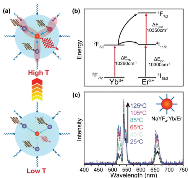
Fig. 6 (a) Thermal activation of phonon-assisted energy transfer. (b) Mismatch of energy levels between \text{Yb}^{3+} and \text{Er}^{3+} ions, illustrating the need for phonon participation in the energy transfer process. (c) Temperature-dependent upconversion emission spectra of \text{NaYF}_4:\text{Yb}/\text{Er} (20/2%) UCNPs (24 nm) in the temperature range of 25–125 °C. Reproduced with permission from ref. 79. Copyright 2014, American Chemical Society.
