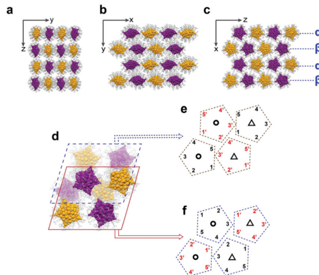
Fig. 2 The self-assembly of \text{Ag}_{70} -TPP clusters on different planes (a) (100), (b) (001), and (c) (010) planes; (d) eight \text{Ag}_{70} -TPP clusters in the same unit cell; (e and f) model diagram of four clusters in the upper and lower layers. (The \text{Ag}_{70} -TPP clusters in two chiral configurations are indicated with different colours. \text{Ag}_{70} -TPP were indicated as pentagons, five phosphine ligands located at the five vertices were numbered and the two poles of the clusters are indicated as \Delta and \circ .)
