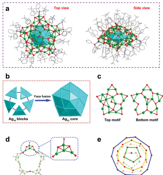
Fig. 1 Structural anatomies of the \text{Ag}_{70} -TPP nanocluster. (a) Top and side views of overall structure; (b) the decahedral \text{Ag}_{23} core; (c) \text{Ag}_{14}\text{S}_{11} , and \text{Ag}_{13}\text{S}_{11} motifs from the side view; (d) the outmost circular \text{Ag}_{20}\text{S}_{20}\text{P}_5 motif; (e) layer-by-layer distribution of S atoms. Color labels: Ag, turquoise/green; S, red; P, magenta; C, gray. For clarity, all H atoms are omitted.
