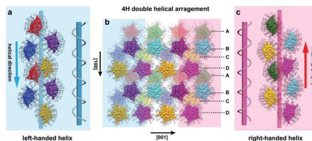
Fig. 3 (a) \text{Ag}_{70} -TPP nanocluster helical arrangement along the [100] direction, (b) double helical 4H arrangement of the \text{Ag}_{70} -TPP nanocluster in the (010) plane, and (c) \text{Ag}_{70} -TPP nanocluster helical arrangement along the [\bar{1}00] direction. (Note: the eight clusters of the same unit cell are labeled in different colors).
