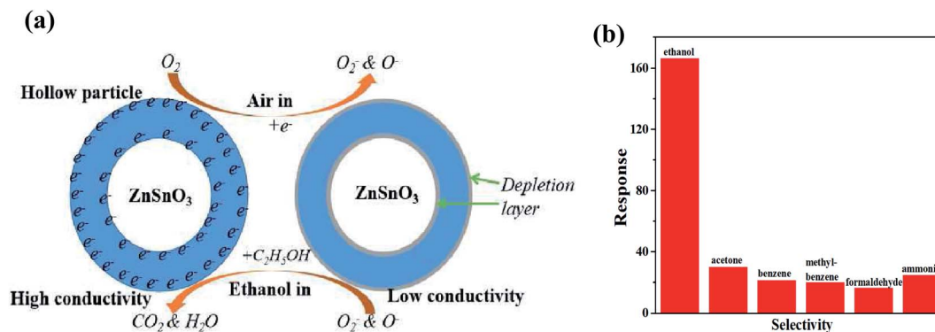
Fig. 17 (a) Ethanol sensing mechanism of \text{ZnSnO}_3 hollow particles. (b) Sensing response ( R_a/R_0 ) of \text{CNT@ZnSnO}_3 exposed to different types of gases, i.e. ethanol, acetone, benzene, methyl-1-benzene, formaldehyde and ammonia (from left to right) 216 (reprinted from ref. 216, Copyright (2020), with permission from Elsevier).
