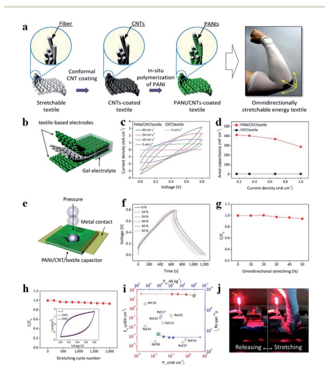
Fig. 1 (a) Synthetic procedure of PANI/CNT. (b) Device configuration of electrochemical capacitors assembled from the textile-based electrode and gel electrolyte. (c) Cyclic voltammetry curves of textile-based electrochemical capacitors under different scan rates. (d) Areal-specific capacitance vs. current density. (e) Schematic illustration of evaluation method for omnidirectional stretchability of PANI/CNT/textile capacitor. (f) Galvanostatic charge/discharge curves at various omnidirectional stretching levels. (g) Capacitance retention under omnidirectional stretching levels. (h) Cycle stability of PANI/CNT/textile capacitors under repeated 20% omnidirectional stretching level. (i) Ragone plot with the previously reported stretchable electrochemical capacitors. (j) LED lighting powered by PANI/CNT/textile capacitors under finger pressure. Reproduced with permission. 14 Copyright 2019, American Chemical Society.
