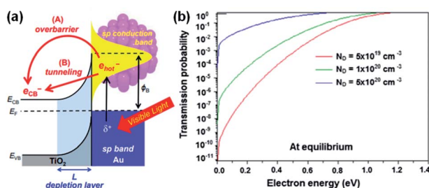
Fig. 8 (a) Band diagram picture of hot electron injection at the Au- \text{TiO}_2 heterojunction by (A) transfer over the barrier or (B) tunneling. Reproduced from ref. 96, copyright 2017, with permission from the Royal Society of Chemistry. (b) Tunneling probability at the Au- \text{TiO}_2 interface as a function of electron energy for different doping concentrations. Reprinted from ref. 90, copyright 2018, with permission from Elsevier.
