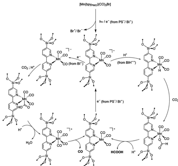
Fig. 17 Proposed mechanisms for the formation of \text{HCO}_2\text{H} and \text{CO} from the photocatalytic reaction with [\text{Mn}(\text{bpy}_{\text{PMO}})(\text{CO})_3]\text{Br} . 116 Reproduced from ref. 116 with permission from the Royal Society of Chemistry.
