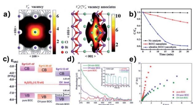
Fig. 13 Schematic representation of the trapped positrons of (a) V_{Bi} defect and V_{Bi}V_O vacancy associates, respectively. (b) Comparison of the photodecomposition of Rhodamine B with ultrathin BiOCl nanosheets and BiOCl nanoplates under simulated solar irradiation. (c) Schematic illustration of the band structure of O_V -rich/poor BOC and pure BOC. (d) Surface photovoltage spectrum of O_V -rich/poor BOC and pure BOC. Current density transients of O_V -rich/poor BOC and pure BOC under visible-light irradiation are shown in the inset. (e) Nyquist impedance plots of O_V -rich/poor BOC and pure BOC. Reproduced with permission from ref. 142 Copyright 2013, the American Chemical Society, and ref. 143 Copyright 2018, The Royal Society of Chemistry.
