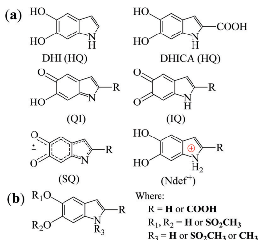
Fig. 1 (a) The building block monomers for non-functionalized melanin. HQ denotes hydroquinone, QI quinone imine, IQ indolequinone and SQ semiquinone. Ndef + is attributed to a charged structure, a synthesis defect. 26 (b) Proposed building blocks of sulfonated melanin. 27
