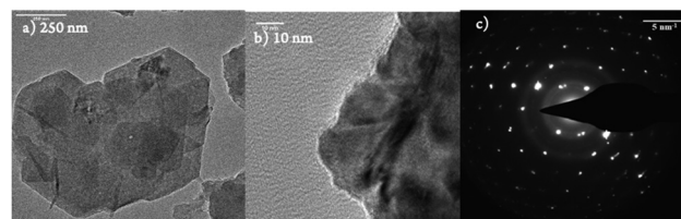
Fig. 2 TEM images (a) and (b). Diffraction of DPCOF spacing which corresponds to 2\theta 18\text{--}19^\circ . The CTM image displays clear hexagonal symmetry and crystalline order which can be seen in DPCOF SAD (c) diffraction from (b).
