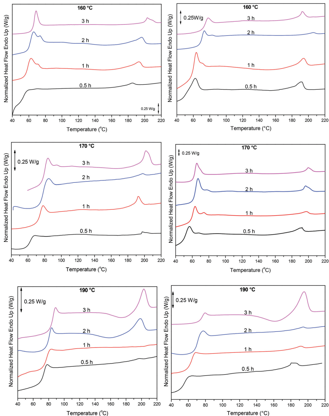
Fig. 10 DSC thermograms of the condensation step at different reaction times and temperatures, catalyzed by Sb 2 O 3 (left) and Sb(CH 3 COO) 3 (right).
