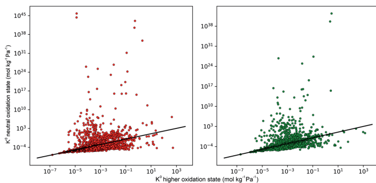
Fig. 2 Comparison of the Henry coefficients for CO 2 (red) and H 2 S (green) in MOFs, predicted by using different sets of partial charges on metal sites. The y -axis corresponds to partial charges calculated using a neutral oxidation state on metal atoms, while the x -axis corresponds to partial charges calculated using a higher oxidation state on metal atoms. A full list of oxidation states may be found in the ESI.†
