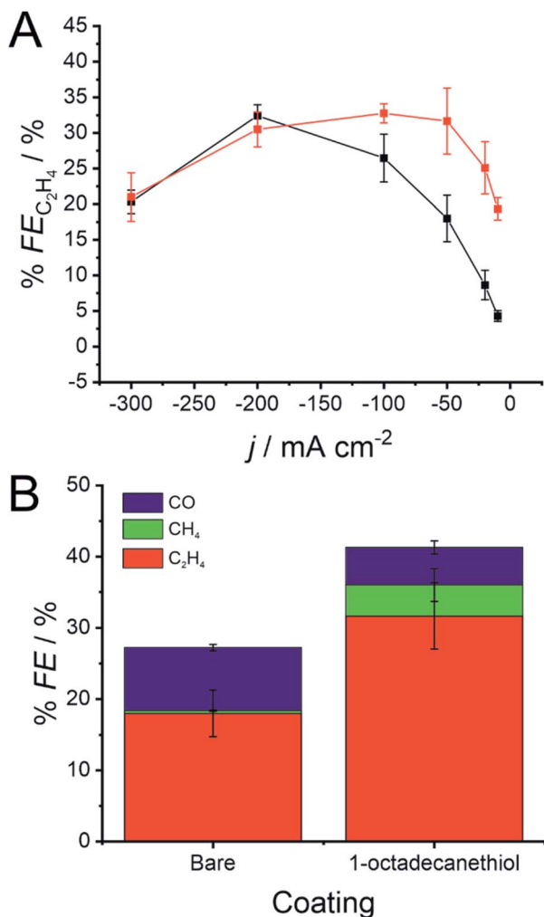
Fig. 4 (A) Faradaic efficiency for \text{C}_2\text{H}_4 formation ( \% \text{FE}_{\text{C}_2\text{H}_4} ) during galvanostatic \text{CO}_2 reduction at a 500 nm Cu GDE in 1 M KOH with (red) and without (black) a monolayer of 1-octadecanethiol to form a hydrophobic interface. (B) % FE for CO, \text{CH}_4 and \text{C}_2\text{H}_4 with and without the 1-octadecanethiol layer during galvanostatic \text{CO}_2 reduction at -50 \text{ mA cm}^{-2} using the same conditions as in (A). Error bars display one standard deviation ( n = 3 ).
