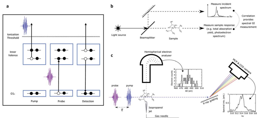
Fig. 1 (a) Experimental methodology for probing hole dynamics in isopropanol. A pump pulse at 502 eV ionizes the molecule, generating inner valence hole (IVH) states. The time delayed probe resonantly interacts with these states via O 1s–IVH transitions, filling the photoexcited hole. This is followed by Auger decay of the core excited cation releasing high energy electrons. (b) General schematic for spectral domain ghost imaging. The incoming source is split into two arms on a shot-to-shot basis. One arm ('pixellated' measurement) provides a reference measurement of the incoming spectrum. The second arm ('bucket' measurement) passes through the sample, and the sample response (such as total photoproduct yield or photoelectron spectrum) is measured. The correlation in the shot-to-shot fluctuations of these two measurements provides the spectral response of the system. (c) Implementation of spectral domain ghost imaging in our experiment. The SASE X-ray pulse passes through a dilute gaseous sample of isopropanol. The 'bucket measurement' is the photoelectron spectrum, measured by a hemispherical analyser. The 'pixellated measurement' is performed by a downstream X-ray spectrometer. Photon depletion through the sample is negligible so the downstream spectral measurement is a faithful measurement of the incoming photon spectrum.
