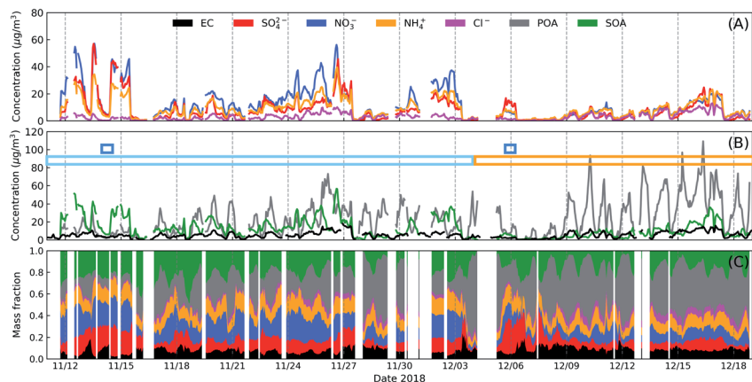
Fig. 2 Time series of submicron aerosol ( PM_1 ) mass concentrations (A and B) and mass fractions of different components (C). In panel (B), the colored rectangles have the same meaning as in Fig. 1. Positive matrix factorization analysis is employed to classify organic aerosol (OA) into various primary OA (POA) factors including hydrocarbon-like OA (HOA), cook-related OA (COA), biomass burning OA (BBOA) and coal combustion OA (CCOA), and a secondary OA (SOA) factor: oxygenated OA (OOA). More details can be found in Fig. 5 and in the work of Sun et al. 19
