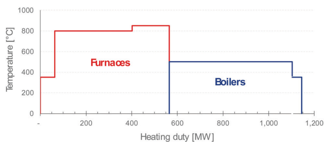
Fig. 4 Typical profile of energy demand of petrochemical plants (furnaces in red and boilers in blue).
