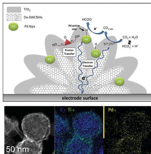
Fig. 6 Top: Graphical sketch of the \text{PdNP/TiO}_2\text{@CNH} nano hybrid and of the interfacial synergy towards the reversible \text{HCOOH} formation; bottom: HAADF (black and white) and EDX elemental mapping of C, Ti and Pd confirming the co-location of the three elements.
