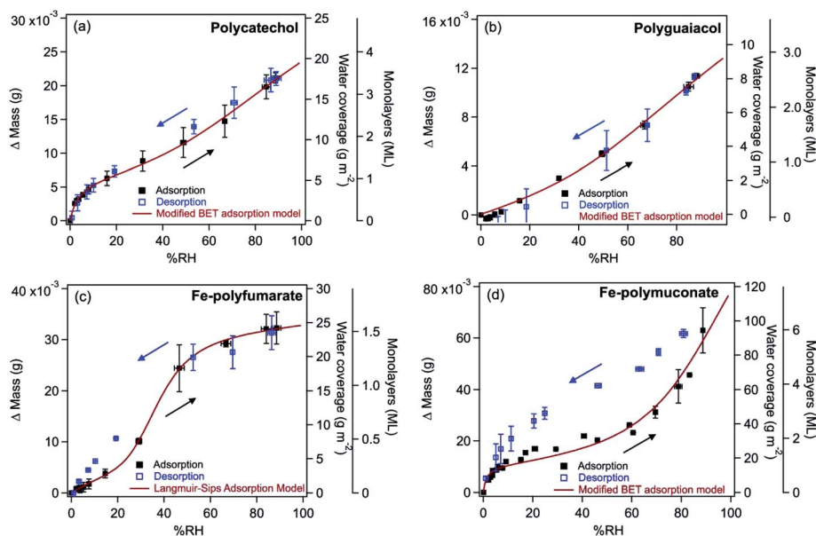
Fig. 33 Water adsorption isotherms at 298 K for (a) polycatechol, (b) polyguaiacol, (c) Fe-polyfumarate, and (d) Fe-polymuconate. The left axis shows \Delta m (g), which is the change in mass due to adsorbed water, as measured using the QCM. The right axes were calculated by converting \Delta m to water mass (g) per surface area ( \text{m}^2 ) of the organic film deposited. The lines through the data represent least-squares best fits to the experimental data using the modified BET and the Langmuir–Sips adsorption models. The outermost right axis was obtained by dividing the water coverage in \text{g m}^{-2} by that at the monolayer coverage obtained from the best-fit parameters (see ref. 307 for details). Reproduced from ref. 307 under the AuthorChoice License from the American Chemical Society, © 2018.
