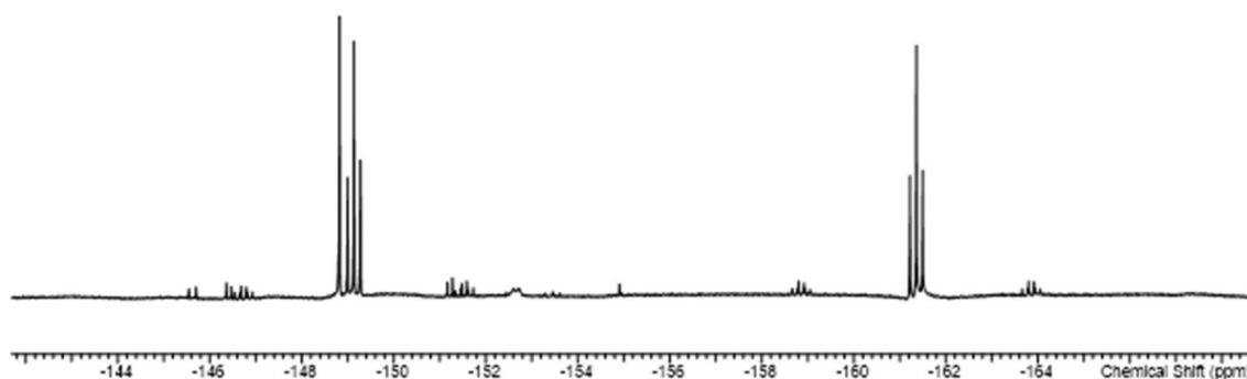
Fig. 6 The ^{19}F\{^1H\} NMR spectrum of [SnF_4(dmsO)_2] (298 K) showing the resonances of the two isomers with ^{117/119}Sn satellites.
