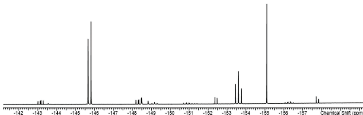
Fig. 7 The ^{19}F\{^1H\} NMR spectrum of [SnF_3(dmsO)_3][OTf] (298 K) showing the resonances of the two isomers with ^{117/119}Sn satellites (the OTf resonance is not shown).
