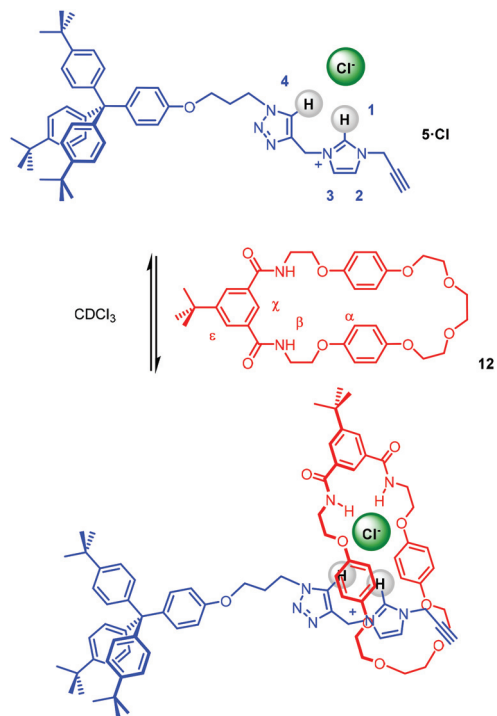
Scheme 3 Pseudorotaxane formation between imidazolium-alkyne thread 5 ·Cl and isophthalamide macrocycle 12 .
