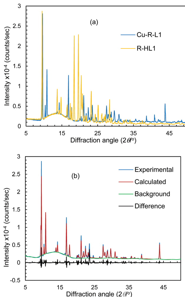
Fig. 5 (a) PXRD patterns for R\text{-HL}^1 and Cu\text{-R-L}^1 . (b) Experimental and calculated Rietveld refinement plots for Cu\text{-R-L}^1 (calculated for \Lambda - Cu\text{-R-L}^1 ; see Fig. S8, S9, ESI † for R\text{-HL}^1 and \Delta - Cu\text{-R-L}^1 ).
