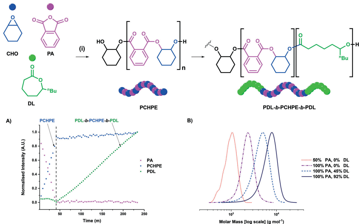
Fig. 3 Switchable polymerization catalysis using PA, CHO and DL utilising complex 1. (i) [\text{Cat}]:[\text{PPNCI}]:[\text{CHD}]:[\text{PA}]:[\text{DL}]:[\text{CHO}] = 1:1:10:100:200:500 , T = 100\text{ }^\circ\text{C} . A) Data from ATR-IR spectroscopy showing the conversion of the different blocks with time. The green series shows formation of PDL, whilst the pink and blue series indicate PA consumption and PCHPE formation, respectively. B) Evolution of polyester molar mass with conversion, from reaction aliquots.
