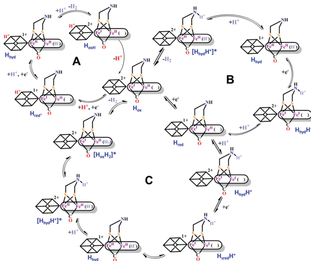
Scheme 22 Proposed catalytic cycles for reversible \text{H}^+ reduction by [FeFe]-hydrogenases. 387–390
