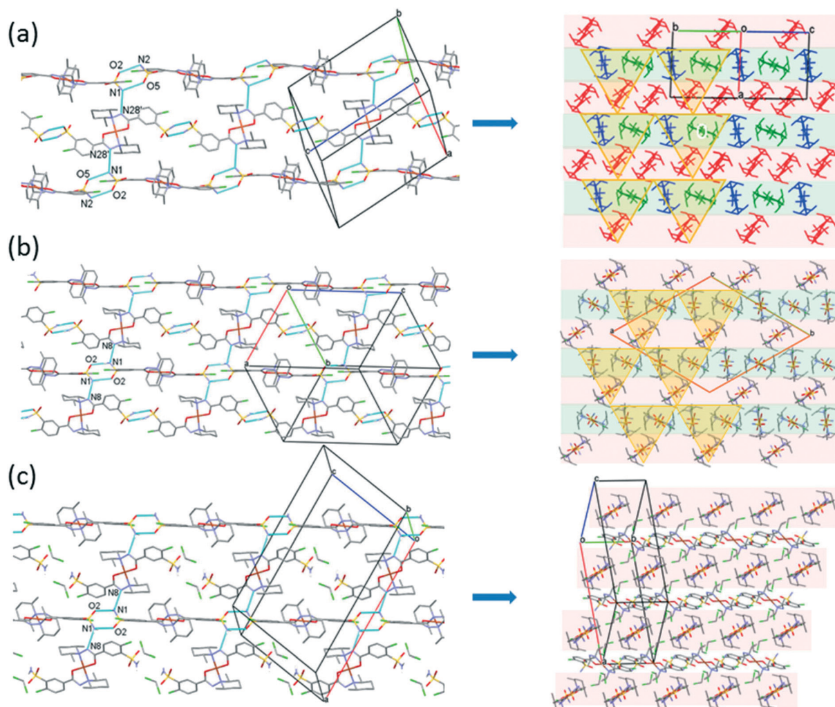
Fig. 11 Packing arrangements in crystal 8 (a) (molecule A is red, B is green and C is blue), crystal 9 (b) and crystal 10 (c) showing the columns formed by N–H \cdots O type hydrogen bonds viewed from the side and also from the top of the columns. The light pink and green colours show the different sheets; the yellow triangles highlight the triangular arrangements of the molecules in the different crystals.
