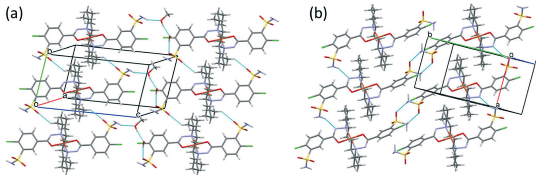
Fig. 10 Analogous packing arrangements in [CuL 2 ] \cdot CH 3 OH \cdot H 2 O crystal 3 (a) and in the solvent-free [CuL 2 ] crystal 7 (b), showing the columns supported by the systems of secondary interactions.
