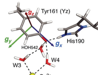
Fig. 7 Orientation and components of the g -matrix for the S_2^{\text{B}}Y_Z^{\bullet} state according to Retegan et al. 182 with DFT-computed values g_x = 2.0054 > g_y = 2.0042 > g_z = 2.0022 . The immediate hydrogen bonding environment of the radical is also depicted.
