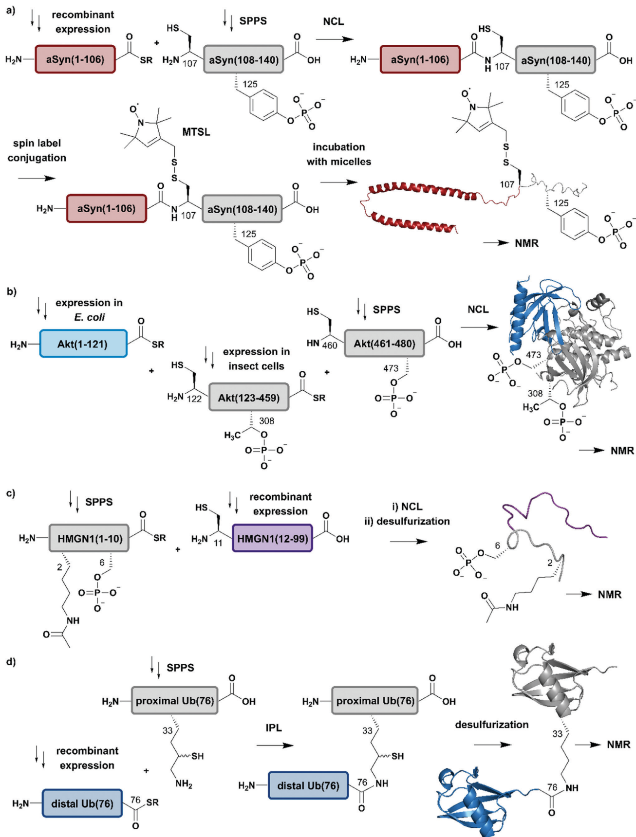
Fig. 4 Expressed Protein Ligation (EPL) for segmental isotope labelling of proteins. (a) Segmental isotope labelling of posttranslationally-modified \alpha Syn(1–140). Recombinant expression of \alpha Syn(1–106) (red) allowed homogenous incorporation of isotopes into the N-terminal \alpha Syn(1–106) segment and chemical
