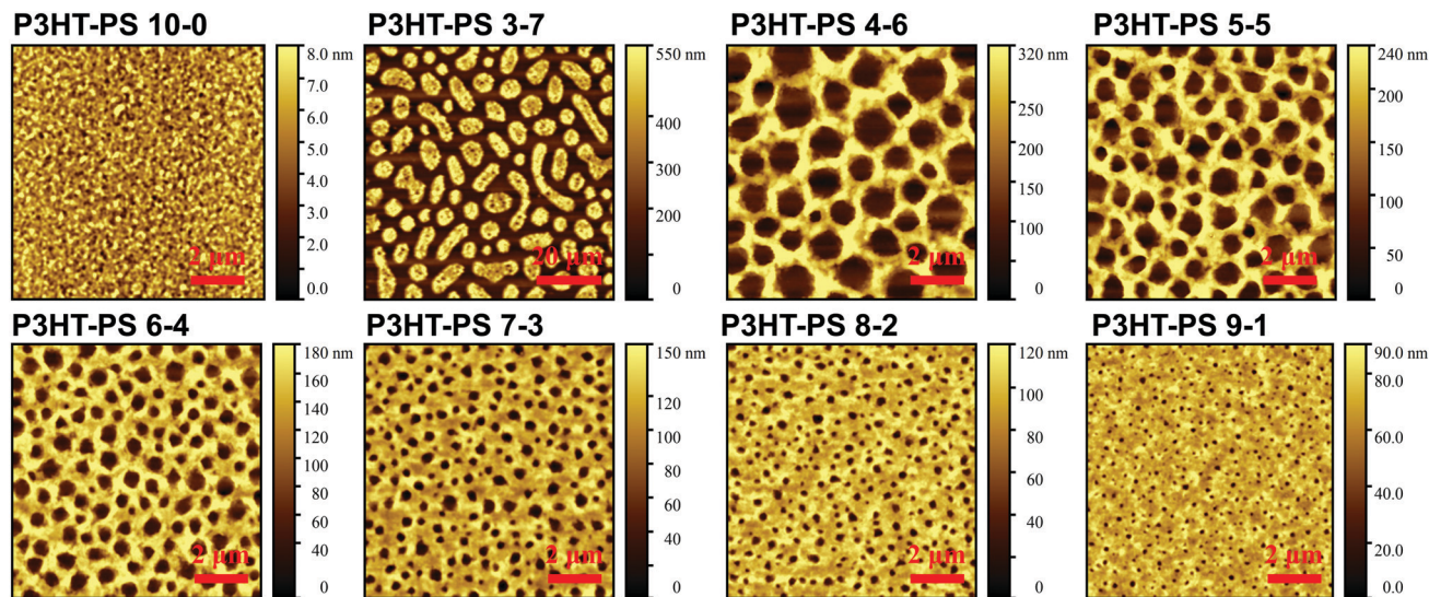
Fig. 2 AFM of the 3D structures produced from phase separation followed by acetone wash with different mixing ratios between P3HT (10 mg ml -1 ) solution and added PS, given in mg ml -1 in chlorobenzene.
