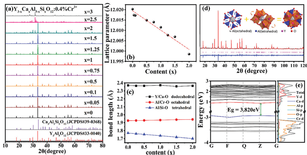
Fig. 1 (a) Powder X-ray diffraction patterns of Y_{3-x}Ca_xAl_{5-x}Si_{2x}O_{12}:0.4\%Cr^{3+} and JCPDS reference data of Y_3Al_5O_{12} and Ca_3Al_2Si_3O_{12} ; (b) lattice constants and (c) ligand bond lengths of Y_{3-x}Ca_xAl_{5-x}Si_{2x}O_{12}:0.4\%Cr^{3+} ( x = 0 to 2) after co-substitution; (d) Rietveld refinement XRD pattern of Y_2CaAl_4SiO_{12}:0.4\%Cr^{3+} . The inset is the structure model of the Ca^{2+}-Si^{4+} co-substituted YAG:Cr; (e) band structure and DOS of Y_2CaAl_4SiO_{12} .
