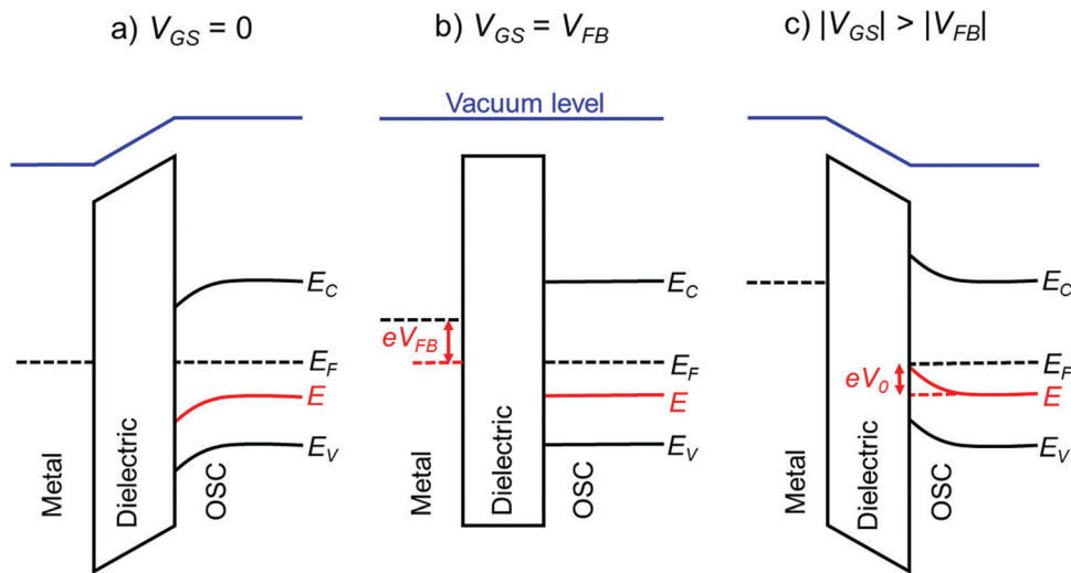
Fig. 9 Energy level diagram at the gate/dielectric/semiconductor interface of an OFET at different gate bias, (a) at V_{GS} = 0 showing initial band bending at the dielectric/semiconductor interface, (b) at V_{GS} = V_{FB} illustrating flat bands and (c) at |V_{GS}| > |V_{FB}| depicting gate-induced band bending. Solid red lines represent an arbitrary trap state for holes, solid black lines the band edges and the broken black lines the Fermi level of the respective material.
