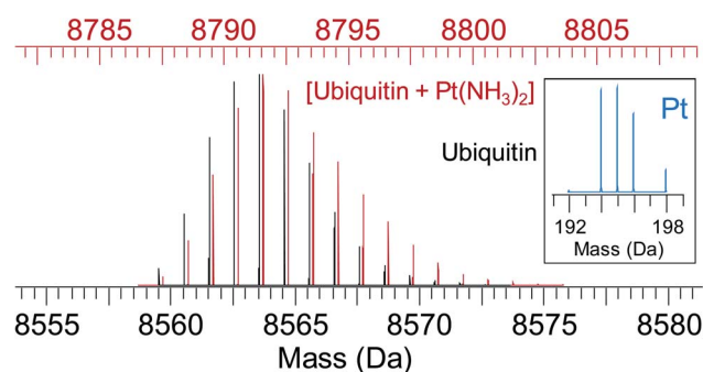
Fig. 5 Simulated isotope pattern for 8.6 kDa protein ubiquitin (black) and [ubiquitin + \text{Pt}(\text{NH}_3)_2 ] (red, shifted by 228 Da, monoisotopic mass of \text{Pt}(\text{NH}_3)_2 , for ease of comparison). Due to the characteristic isotope pattern of Pt (inset), the isotopic distribution of the protein-metal complex is broader and shifted to higher mass compared to the apo-protein. Automated peak-picking procedures can identify such platinated species in complex mixtures ( e.g. cell lysates) providing insight into the binding sites for metallodrugs on proteins. 119
