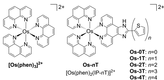
Chart 1 Molecular structures of reference compound [Os(phen) 3 ] 2+ and Os-0T–Os-4T. The chloride salts were used unless otherwise specified. The compounds were racemic mixtures of the \Delta/\Lambda isomers.
