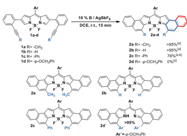
Scheme 2 Scope of the cycloisomerization of 1 to form 2 with different substituted alkynes. [a] Yields were determined after purification using a chromatography column. [b] 20% \text{PPh}_3\text{AuCl}/\text{AgSbF}_6 , 40 °C, DCE and 1 h. [c] not detected, and 2d' was quantitatively obtained.
