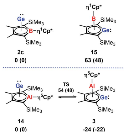
Fig. 8 Relative energies \Delta E and relative free Gibbs enthalpies at T = 298 \text{ K} \Delta G^{298} (in brackets) of isomeric borole 2c and alumole 14 complexes and germa complexes 15 and 3.
