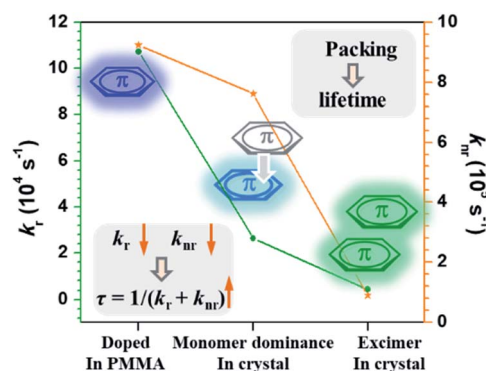
Fig. 5 Changing tendency of the fluorescent radiative rate ( k_r ) and non-radiative rate ( k_{nr} ) for CS-2COOCH 3 in different states.
