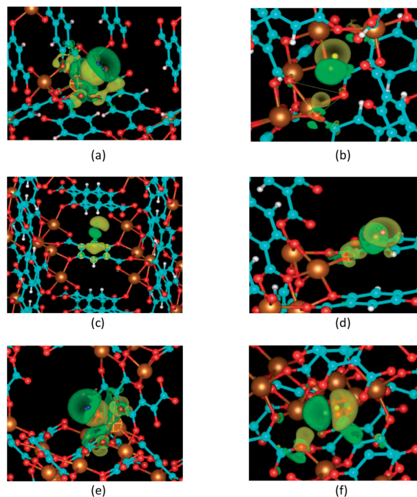
Fig. 4 Iso-surfaces of the electron density deformations upon hydrogen adsorption onto (a) P 1 , (b) P 2 , (c) P 3 and (d) P 4 sites in the BDC-based Mg-MOF-74 framework, (e) P 1 and (f) P 2 sites in the DHF-based Mg-MOF-74 framework. The isovalues is 0.0001|e| Å -3 . Yellow and green denote electron donated and loss surfaces respectively. Red, brown, cyan and white spheres represent oxygen, magnesium, carbon and hydrogen atoms of the frameworks respectively. P 1 , P 2 , P 3 and P 4 hydrogen molecules in the BDC-based framework are represented by blue, yellow, green and pink spheres respectively. P 1 and P 2 hydrogen molecules in the DHF-based framework are represented by blue and pink spheres respectively.
